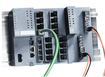
SCALANCE XM416-4C + PE400-8SFP
