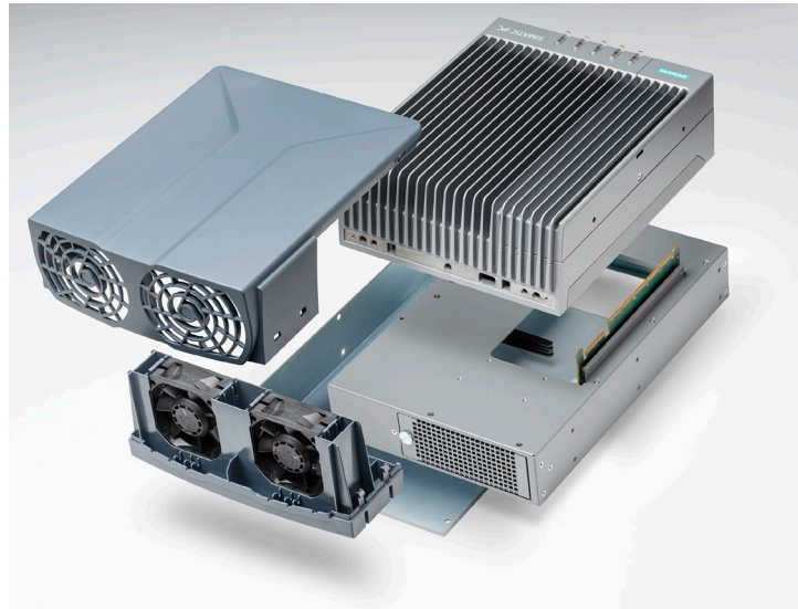
SIMATIC IPC BX-59A
